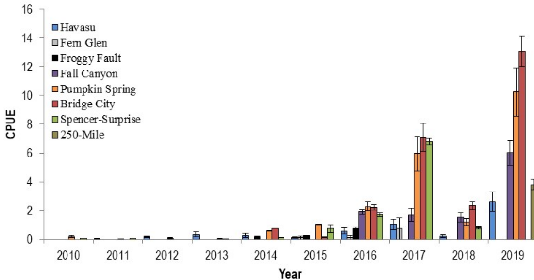
Figure 6. Mean CPUE \pm 95% CI, captures per overnight hoop net) of adult humpback chub Gila cypha ( \geq 200 mm TL) for sampling reaches from Havasu downriver 2010-2019. Approximate river miles for each site are as follows: Havasu (155.8-159.2), Fern Glen (168.5-172.5), Froggy Fault (196.0-198.5), Fall Canyon (210.2-213.9), Pumpkin Spring (212.5-216.0), Bridge City (236.6-238.7), Spencer-Surprise (245-249.5), and 250-mile (249.7-252.5). Note: The 250-mile reach was not sampled until 2019.
