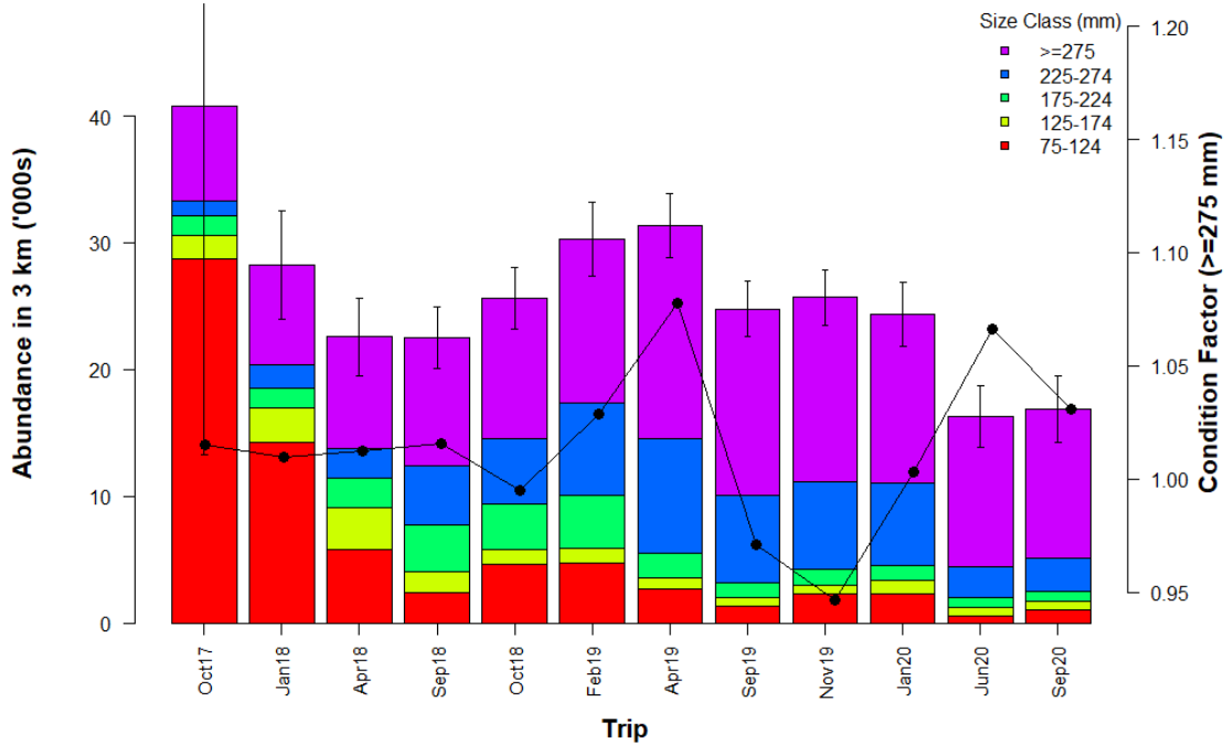
Figure 6. Rainbow trout abundance estimates (stratified by 5 size-classes) in the lowest sub-reach 1C during the Trout Recruitment and Growth Dynamics sampling period in Glen Canyon, AZ. Size classes are assigned by fork length, 75-124 mm, 125-174 mm, 175-224 mm, 225-274 mm, and > 275 mm. The secondary line graph represents the relative condition of trout ≥ 275-mm FL in sub-reach 1C.
