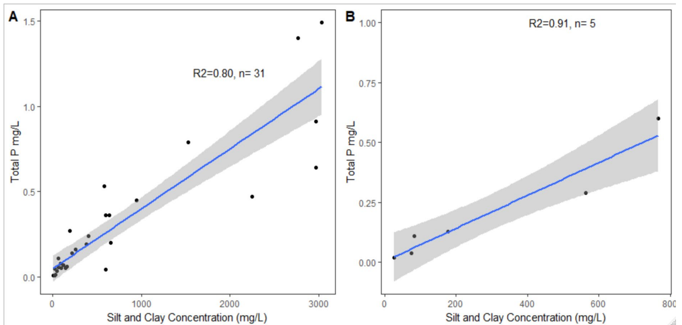
Figure 4. Physical silt and clay measurements predict total phosphorus (TP) concentrations at two long term gage sites on the Colorado River: the Colorado River upstream of Diamond Creek (panel A, gage 09404200) and the Colorado River near Phantom Ranch (panel B, gage 09402500). Measurements at the Colorado River upstream of Diamond Creek (river mile 224) were taken between 1989 and 2019. Less data is available at the Colorado River near Phantom Ranch (river mile 89) and ranges from 2014-2019. Preliminary data, subject to revision.
