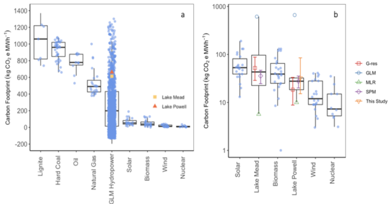
Figure 4. Panel a: Adaptation from Figure 2 of Scherer and Pfister (2016): Carbon footprints of various energy sources. The dots show all values included for each source (although only the 10th and 90th percentile of systems are shown for GLM hydropower to improve visualization). The boxes show upper and lower quartiles (25% and 75%), and the horizontal line indicates the median. The whiskers extend to the largest values no more than 1.5 * the IQR. Panel b: the renewable energy subset of panel a, plotted on a log scale and including the multiple carbon footprint estimates for Lake Powell and Lake Mead estimated by our modeling efforts. Color and shape of the marker indicates the source of the carbon footprint estimate for Lake Powell and Lake Mead. SPM refers to the surface productivity model (DelSontro and others, 2018), MLR refers to multiple linear regressions (Hertwich, 2013), GLM refers to generalized linear modeling (Scherer and Pfister, 2016), and G-res refers to the G-res too (Prairie and others, 2017). Whiskers indicate model or measurement 95% CI range.
