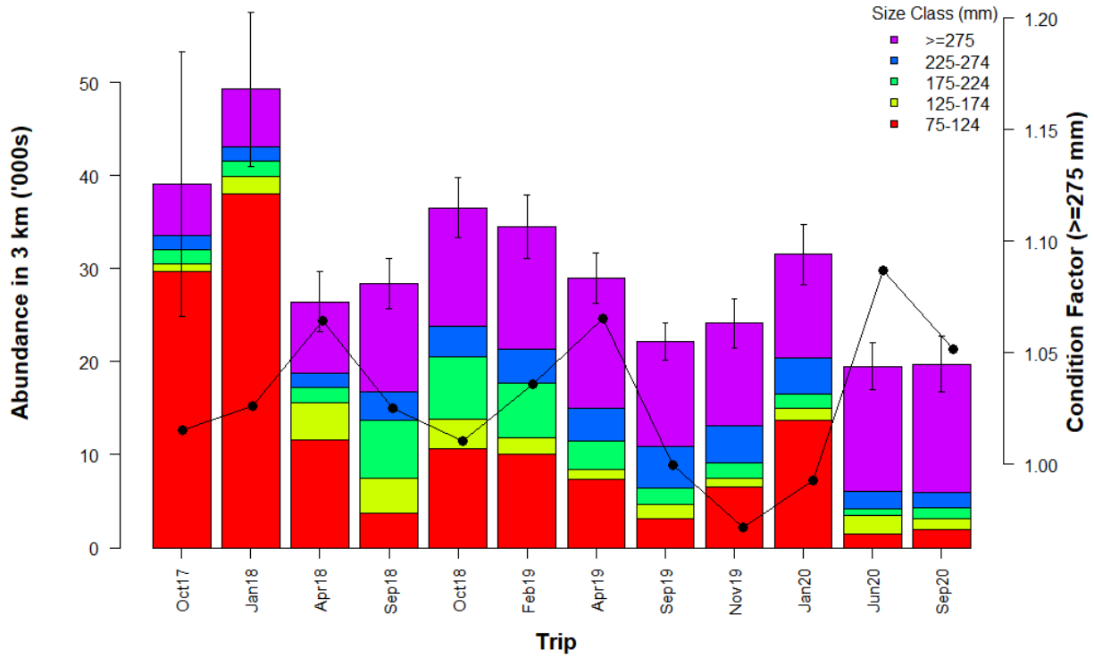
Figure 5. Rainbow trout abundance estimates (stratified by 5 size-classes) in the middle sub-reach 1B during the Trout Recruitment and Growth Dynamics sampling period in Glen Canyon, AZ. (Note that this sub-reach will be eliminated from the future sampling design as per FY 2021-23 TWP.) Size classes are assigned by fork length, 75-124 mm, 125-174 mm, 175-224 mm, 225-274 mm, and > 275 mm. The secondary line graph represents the relative condition of trout \geq 275 -mm FL in sub-reach 1B.
