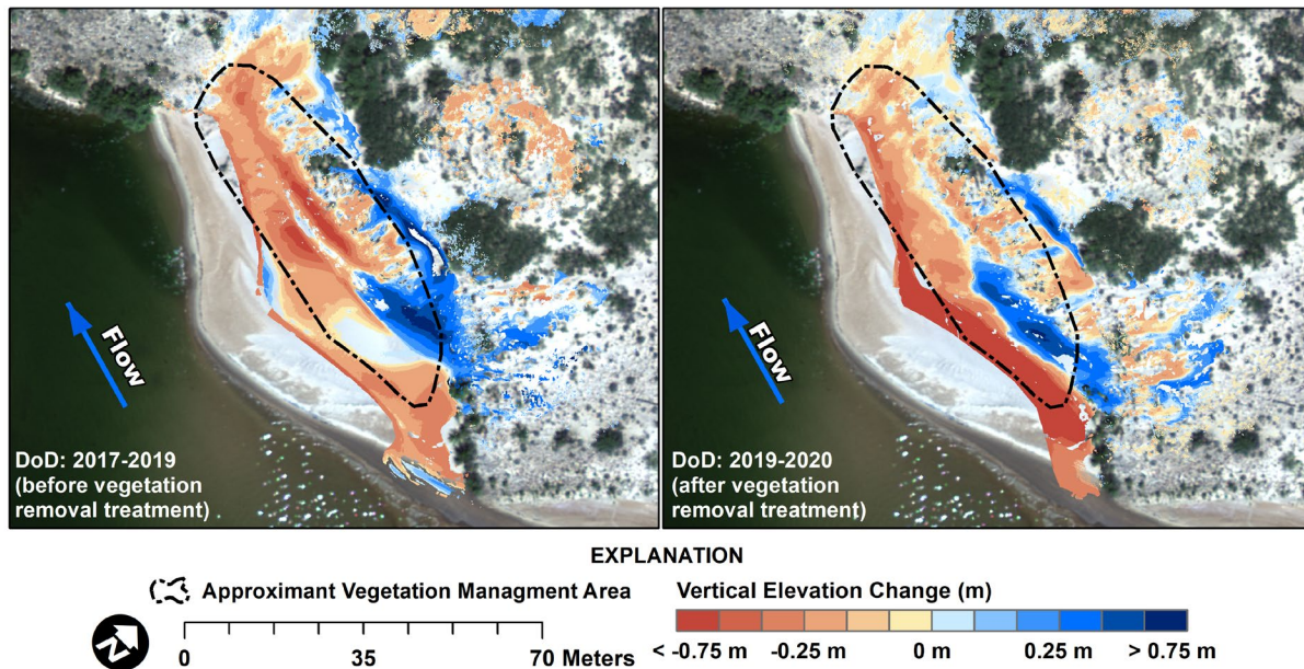
Figure 1. Photos and lidar survey data showing the vegetation removed by the National Park Service during an experimental vegetation management treatment near archaeological site AZ:C13:0321. The treatment at this and other sites is intended to increase sediment storage at the sites by enhancing aeolian transport of Colorado River sand deposited during high-flow experiments from sandbars to archaeological sites. Vegetation removal at this location exposed an aeolian dune that is visible in the photos and lidar data. In the lidar data panels (bottom images, previous page): the grey pixels are the sandy ground surface, and the colored pixels are vegetation; the vegetation pixel colors are scaled by plant canopy height, where cool colors are shorter plants and the warmer colors are taller plants. In the lidar-derived topographic change detection maps (images above), the colored pixels show erosion and deposition of sediment that occurred on the aeolian dune that is derived from and superimposed on the river sandbar at the location.
