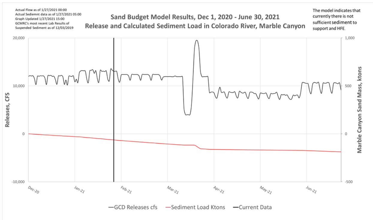
Figure 2. Sand budget model results from January 27, 2021. The spring disturbance flow is projected to export an additional 26,000 metric tons relative to normal operations.
