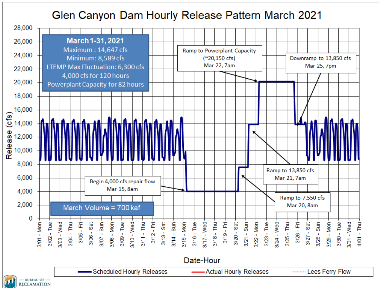
Figure 1. Spring disturbance flow hydrograph that is recommended for implementation in March 2021.
