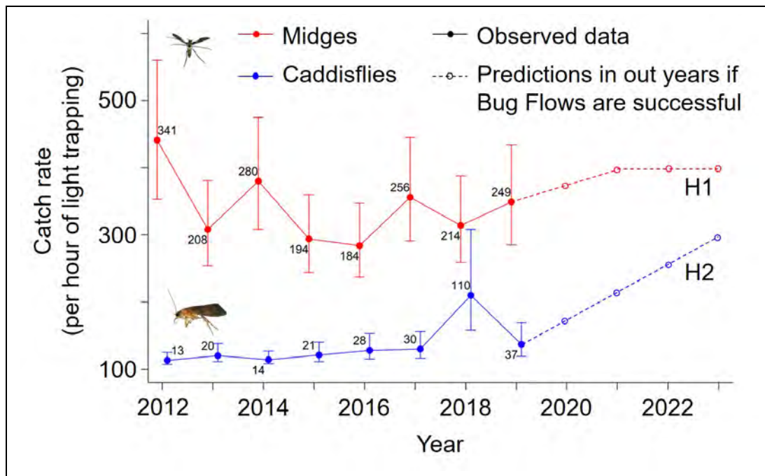
Figure 2. Citizen science light trap catches of midges and caddisflies by year (solid lines and circles) and predicted future catch rates (H1 and H2) based on Bug Flows modeling (dashed lines and circles).
