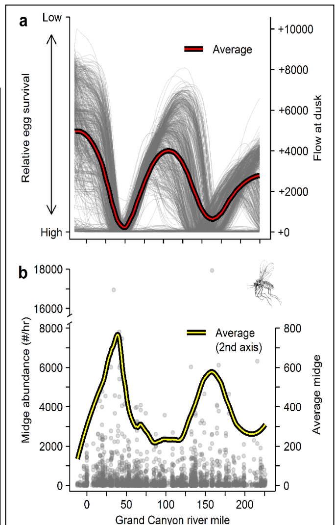
Figure 3. The timing of hydropeaking waves determines insect abundance in Grand Canyon. Hydropeaking waves released from the Dam propagate downstream, and at river miles 50 and 165 daily flow minima occur at dusk when insect egg laying occurs (a). Midge abundance peaks at these same river miles, because of variability in egg survival, with average abundance more than three times greater at locations where the daily flow minima coincide with peak egg-laying activity (b). Adapted from Kennedy and others (2016).
