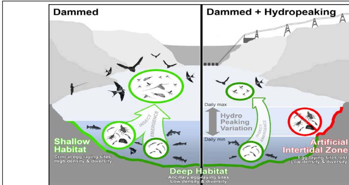
Figure 1. Conceptual model of how hydropeaking affects aquatic insects. Aquatic insects are ubiquitous in freshwaters and are the primary prey for myriad species of wildlife living in and along rivers. These insects have complex life cycles that include a terrestrial winged adult life stage, whereas egg, larval, and pupal stages are aquatic. Ecologically important insect groups such as mayflies, stoneflies, and caddisflies cement their eggs along river-edge habitats, making them especially sensitive to hydropeaking and other dam water management practices that affect these edge habitats.
