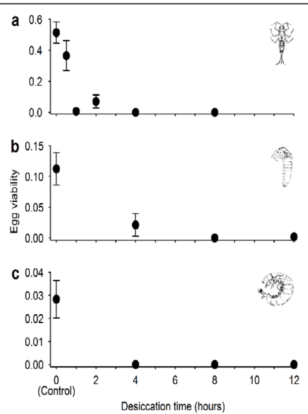
Figure 2. Aquatic insect eggs die after short periods of drying, such as along the banks of a hydropeaking river. Graph shows egg viability (number of hatched eggs/total eggs) after desiccation for eggs of (a) a type of mayfly ( Baetis sp.), and two types of caddisfly (b: Brachycentrus ; c: Hydropsyche ). Adapted from Kennedy and others (2016).
