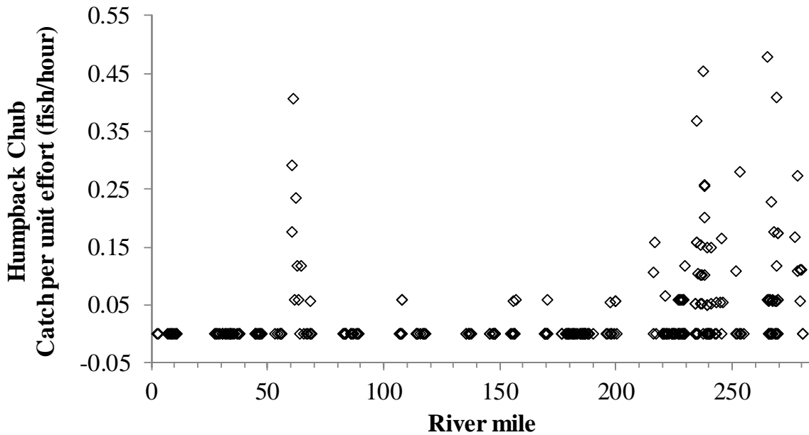
Figure 2. Catch per unit (fish/hour) of humpback chub captured via baited hoop nets (n=319) in 2016 by river mile (RM) from Arizona Game and Fish Department system wide sampling of the Colorado River from Lees Ferry (RM 0 to Pearce Ferry Rapid RM 281.4)
