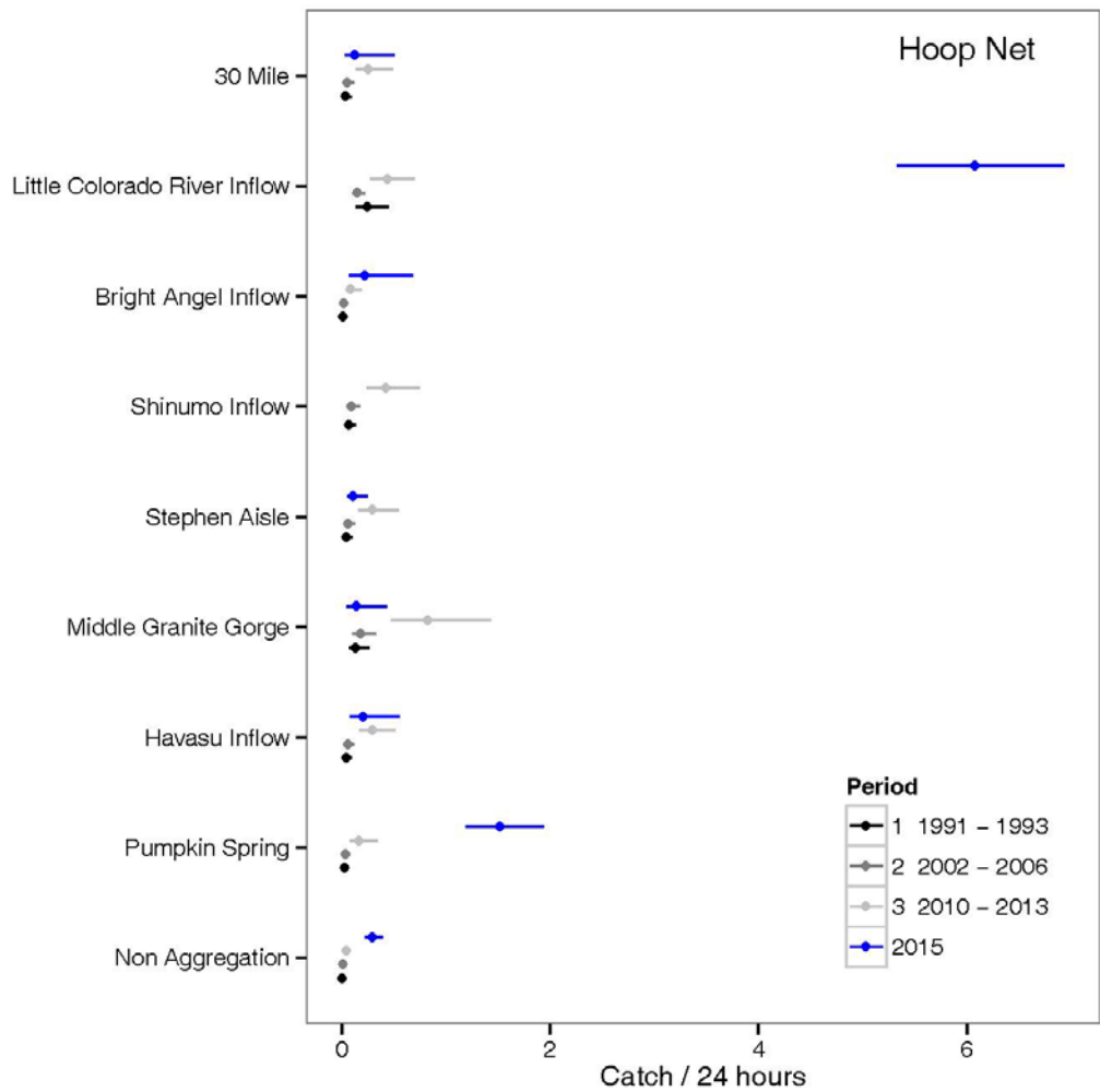
Figure 1. Catch per unit effort index of humpback chub captured in hoop nets from 1991-1993, 2002-2006, 2010-2013, and 2015. Note, 2016 data is still being analyzed.
