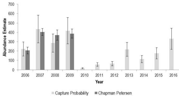
Figure 2. Abundances ( \pm 95\% CI) of adult humpback chub in lower reach downstream of Chute Falls (rkm 13.6 – 14.1) since summer 2006. Note, abundances for both above and below Chute Falls are shown as those estimated with Chapman Petersen mark-recapture (dark grey bars) and those estimated using capture probability data (light grey bars) derived from the 2006-2009 Chapman Petersen mark-recapture efforts.
