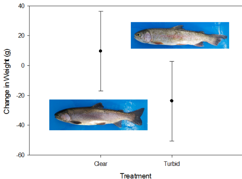
Figure 5. Effects of low level turbidity (<50 FNU) on rainbow trout as measured by mean change in weight during a 30-day laboratory trial. Error bars indicate 95% confidence intervals around the mean change in weight.
