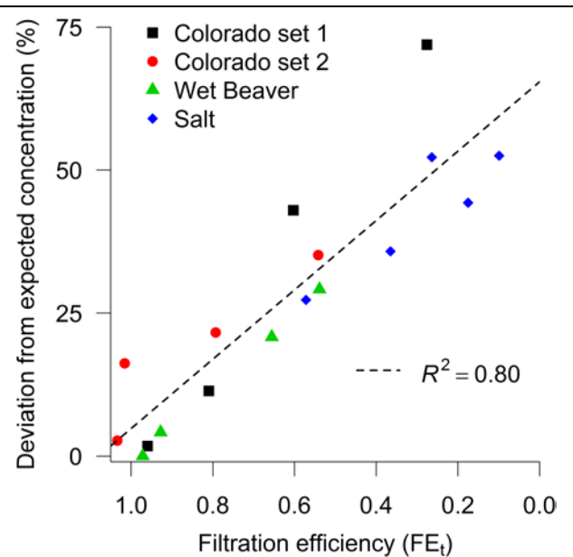
Figure 5. Graph showing the relationship between filtration efficiency of drift nets (a measure of clogging) and the reliability of drift concentration estimates. A filtration efficiency of 1 represents an unclogged drift net. Adapted from Muehlbauer and others (In press).
