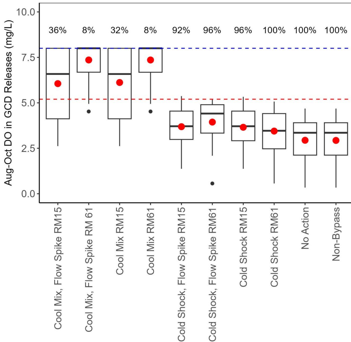
Figure 3-50 Mean August to October DO Concentrations in Glen Canyon Dam Outflows*
