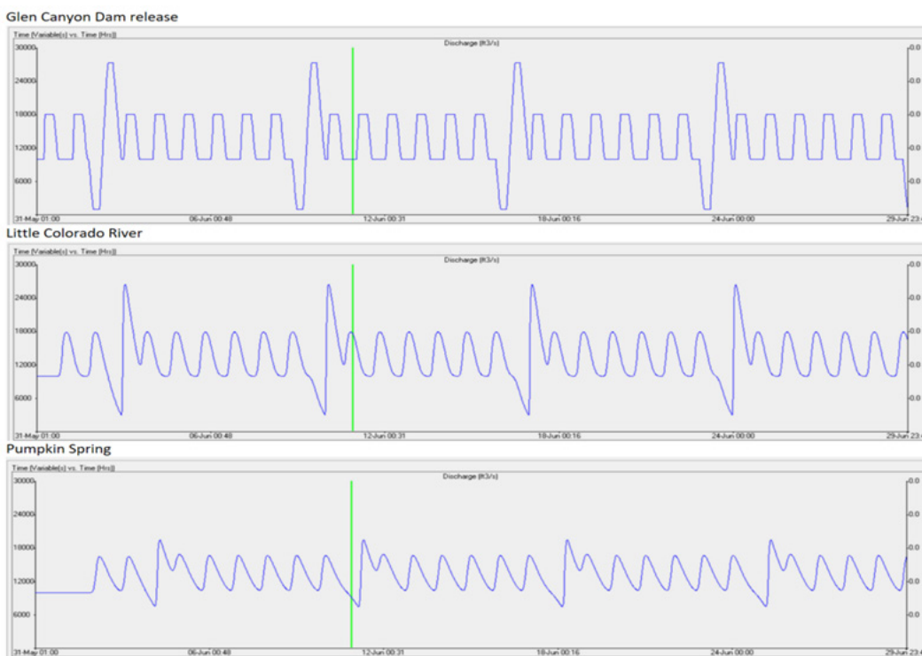
Figure 2-6 Non-Bypass Alternative Flow Modeling of “Collapsing” Trough
